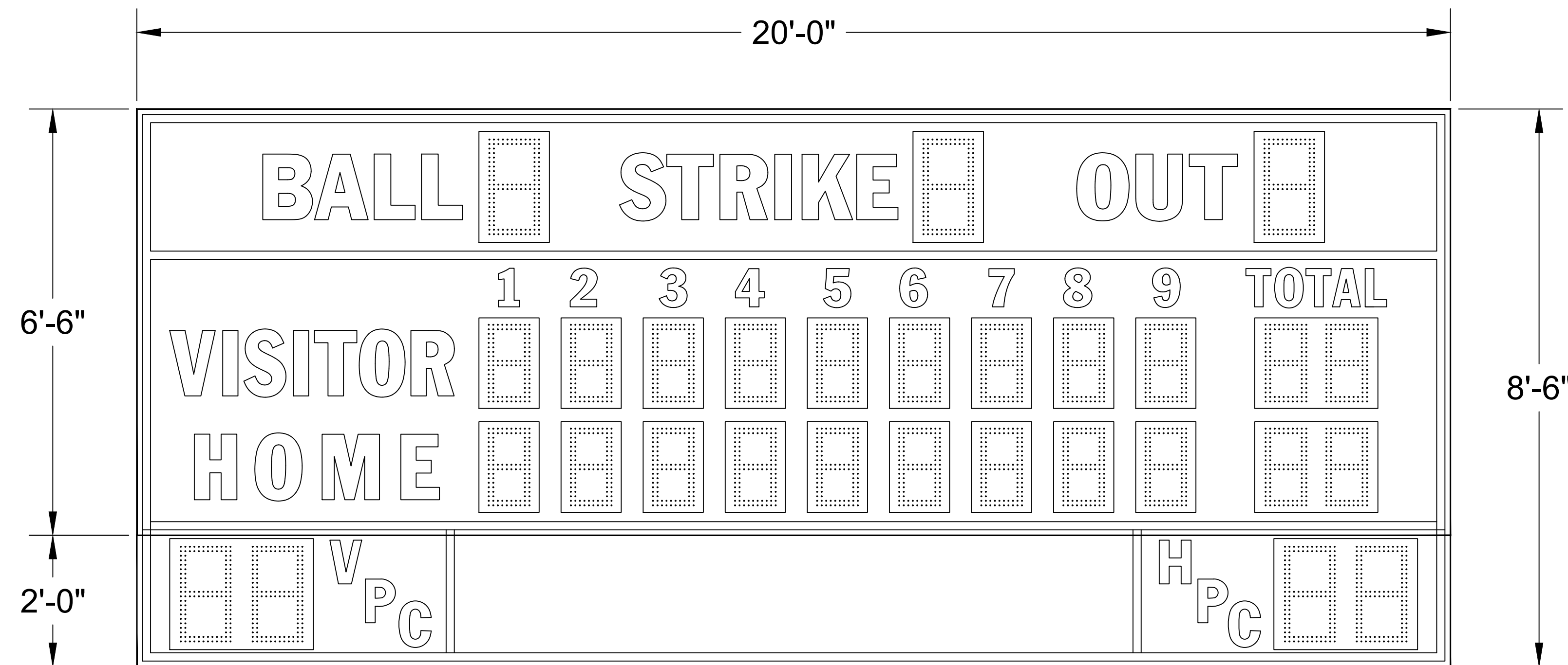
BA-7120PC-2 (18"H DIGITS MOVED TO ENDS OF PITCH COUNT SECTION, ADDED TRIM)
